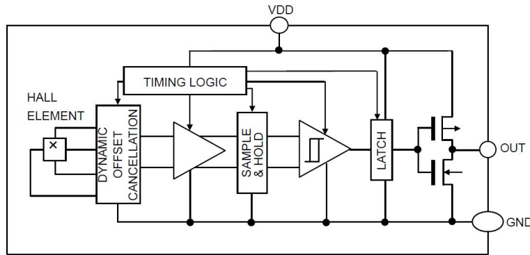
Figure 2, Block Diagram of AS1853
