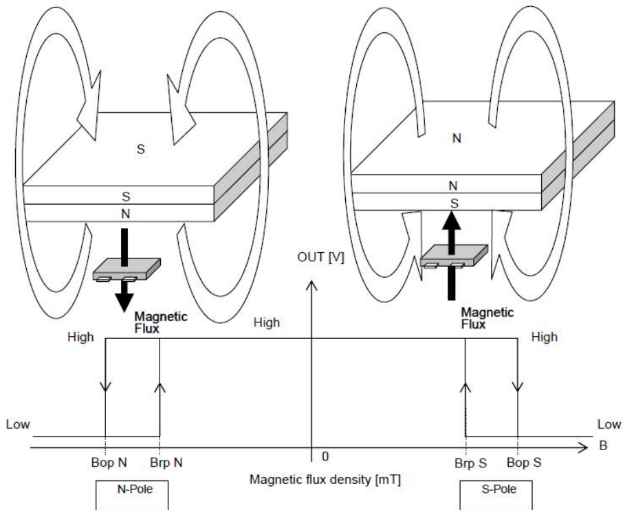
Fig 3, Magnetic Operation Characteristic of AS1853
